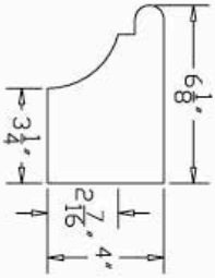
SIDE VIEW SCALE 1/4" = 1"
