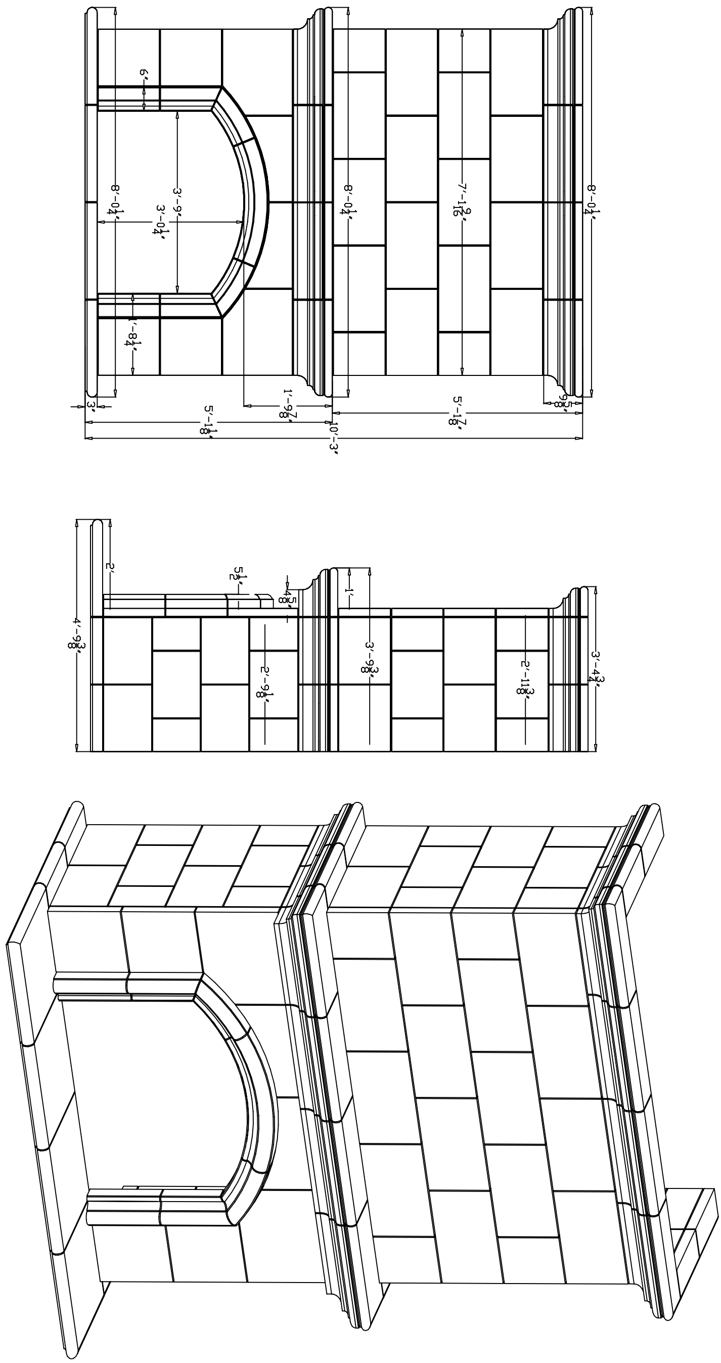
FRONT VIEW SCALE 1/2"=1'
