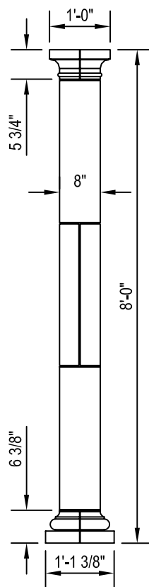
FRONT VIEW
