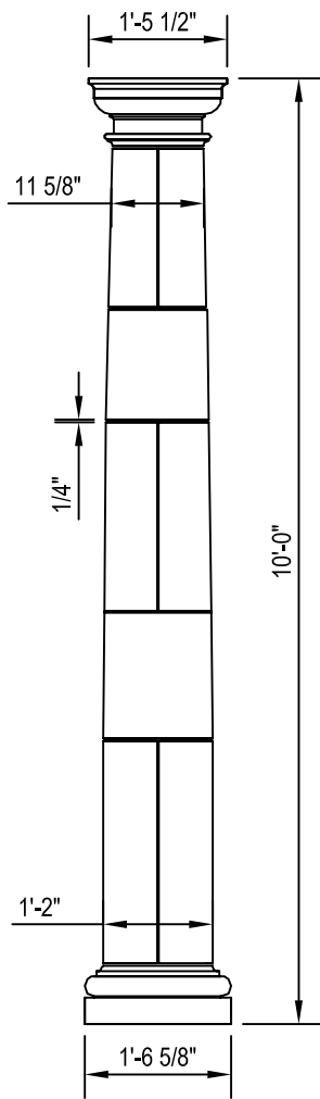
FRONT VIEW
