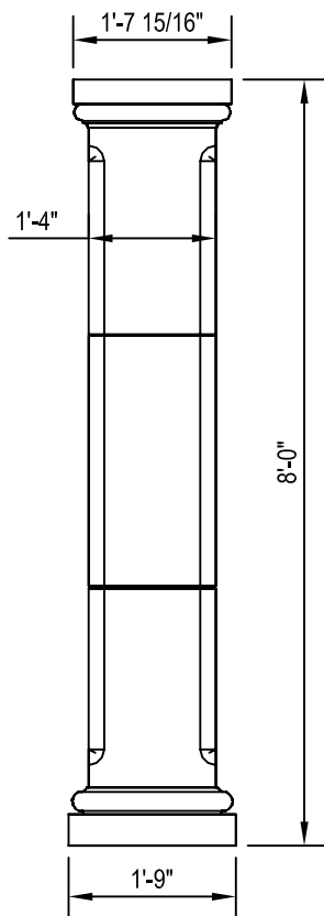
FRONT VIEW
